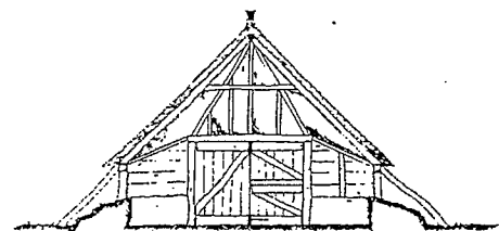
DWARSDOORSNED
